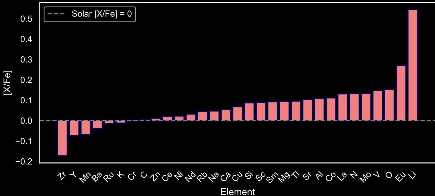
Abundance Pattern for GALAH Star Field [112] (N=217)
