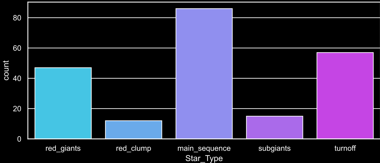
Field [112] Count plot of Star Type
