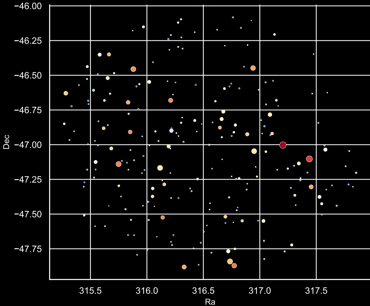
Field [112] Ra [316.45] Dec [-47.03] Stars: 217
