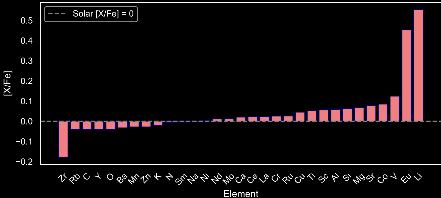
Abundance Pattern for GALAH Main Sequence Stars: Star Field [112] (N=86)
