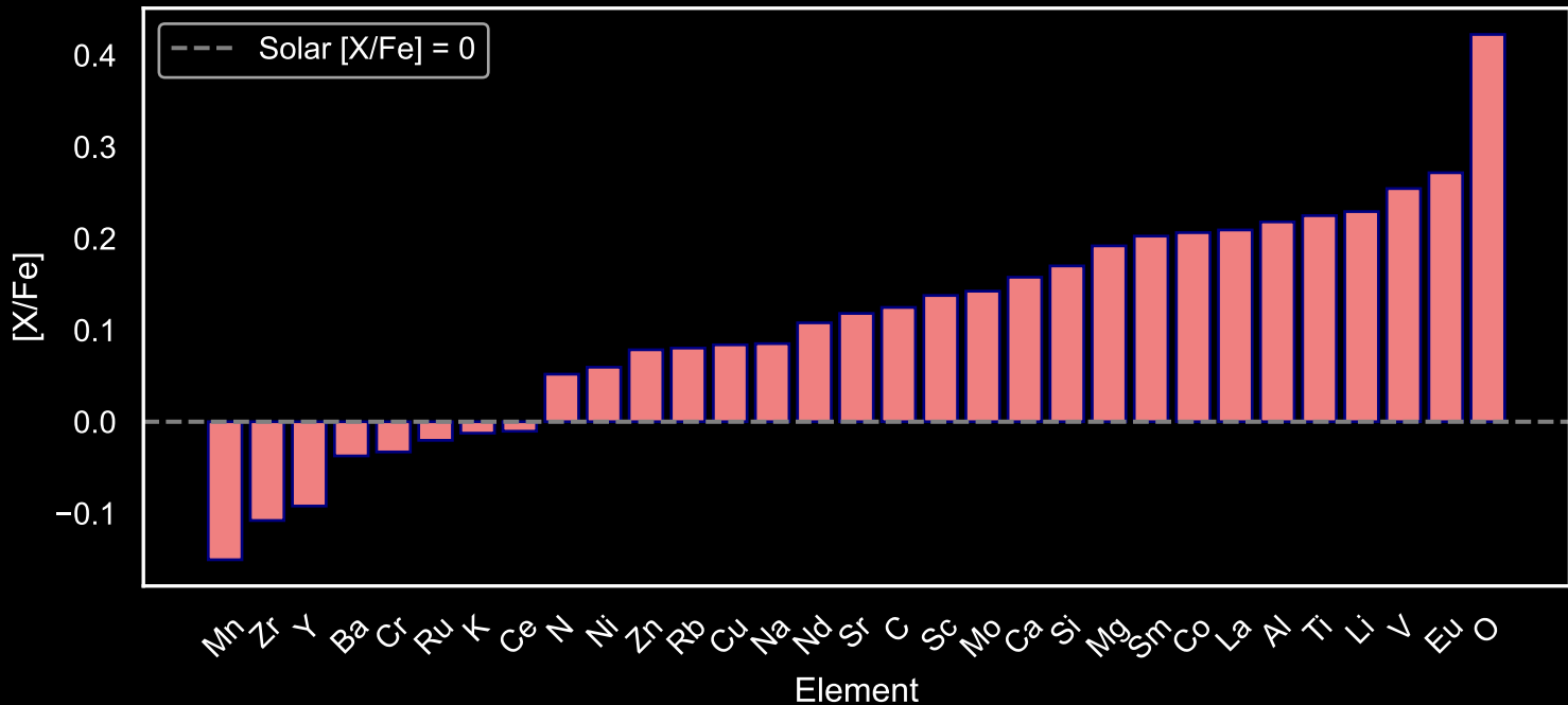
Abundance Pattern for GALAH Red Giants: Star Field [112] (N=59)
